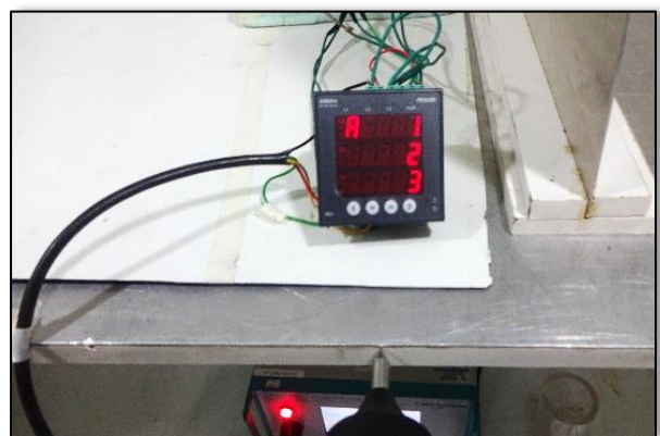
Indirect Discharge on VCP and HCP Test Setup Photos
