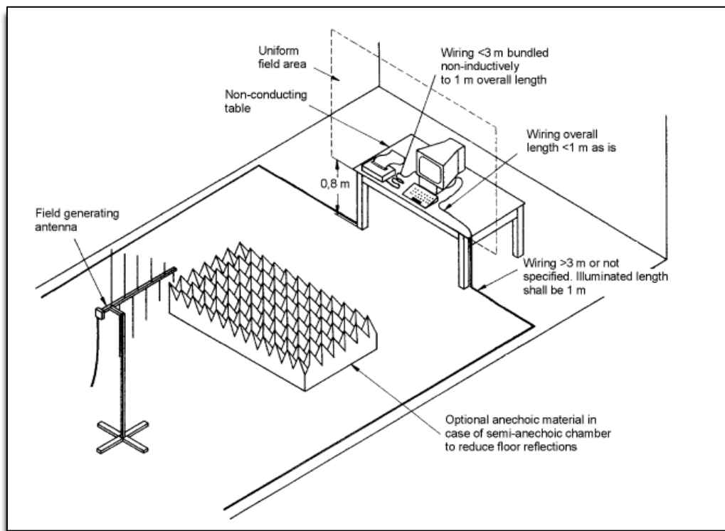
Figure 8: Radiated immunity Test Setup
