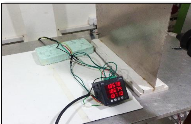
Indirect Discharge on VCP and HCP Test Setup Photos
