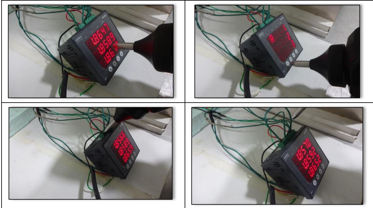
Air Discharge on EUT Test Setup Photos
