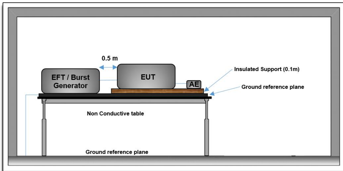
Figure 14: Electrical Fast Transient Test Setup
