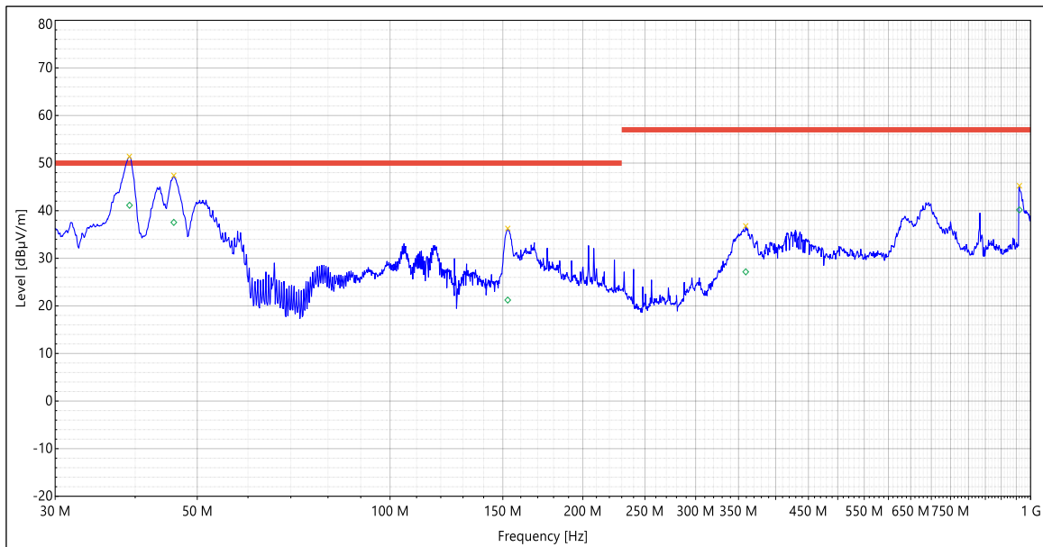
Graph 2: RE_ 30MHz to 1GHz_ Vertical
