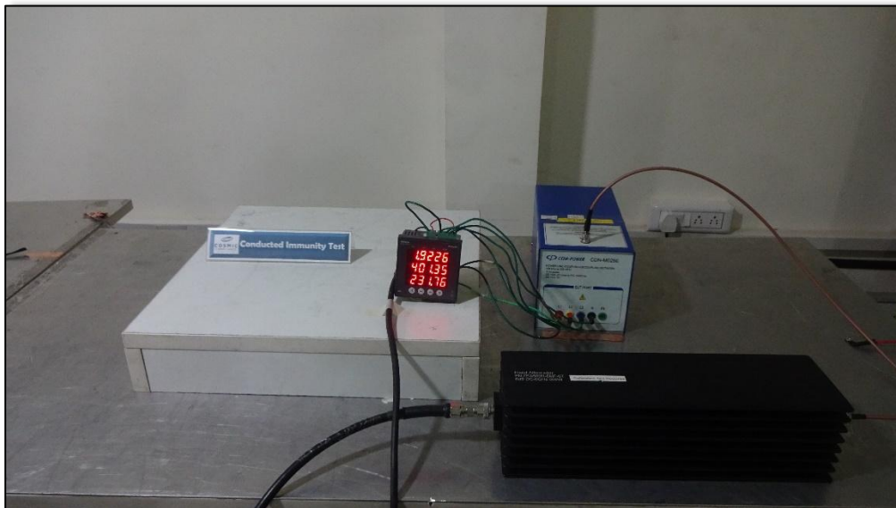
Figure 19: Test Setup Photos
