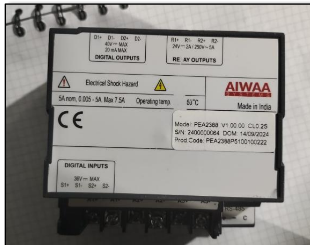
Figure 2: Marking Label of EUT
