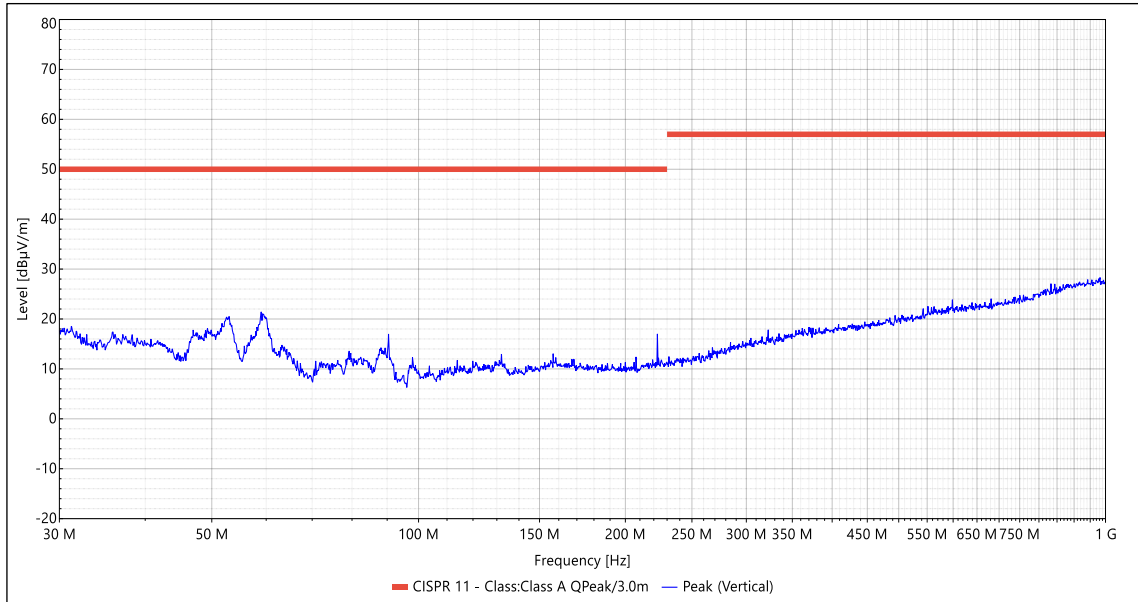
Graph 1: RE_ 30MHz to 1GHz_ Ambient
