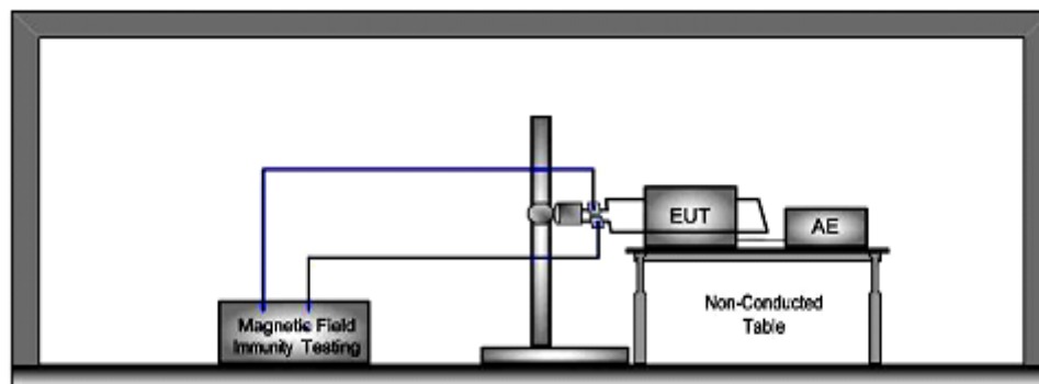
Figure 20: PFMF Test Setup
