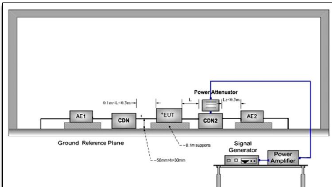
Figure 18: Conducted Immunity Test Setup
