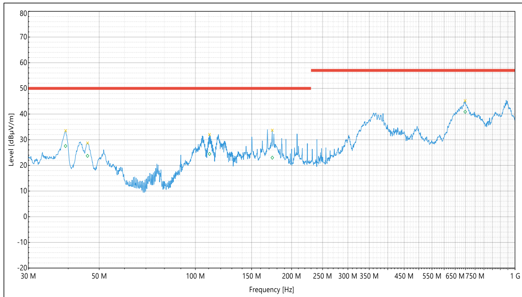
Graph 3: RE_ 30MHz to 1GHz_Horizontal
