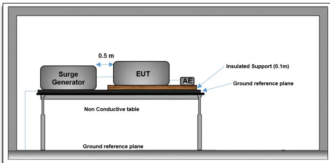
Figure 16: Surge immunity Test Setup
