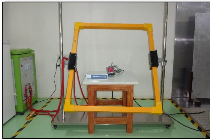
Test setup photograph of Z axis
